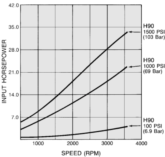
H90 Horsepower/Speed
